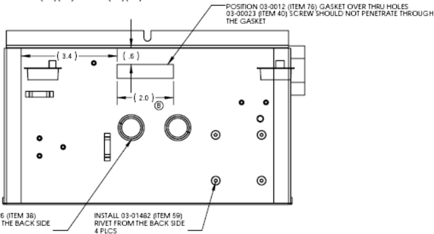
ELECTRICAL BRACKET DETAIL
